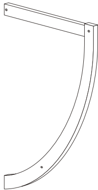
①x1 50x2.5x1.4cm
