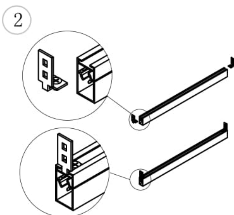
Install the metal front rail using the metal bracket
